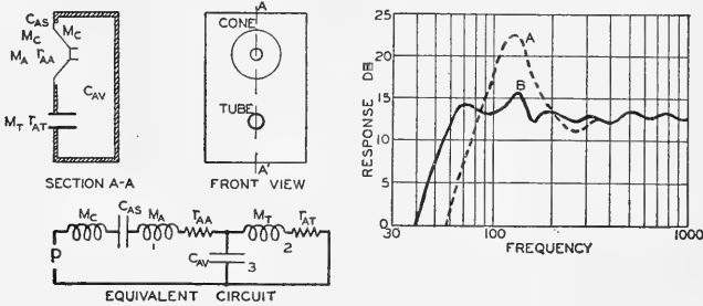
FIG. 7.11. Phase inverter loud speaker and the equivalent circuit of the acoustical system. M_C the inductance of the cone. C_{AS} the acoustic capacitance of the suspension system. M_A and r_{AA} the inductance and the resistance of the air load upon the front of the cone. C_{AV} the acoustic capacitance of the cabinet volume. M_T and r_{AT} the inductance and acoustic radiation resistance of the tube. The pressure p of the generator in the acoustical system is the force generated in the voice coil divided by the area of the cone. The pressure response frequency characteristic of the phase inverter loud speaker is labeled B on the graph. The pressure response frequency characteristic of a loud speaker in a typical cabinet having the same volume as the phase inverter is labeled A on the graph. (After Dickey, Caulton and Perry.) (Courtesy of The Blakiston Company from Olson and Massa, "Applied Acoustics.")
